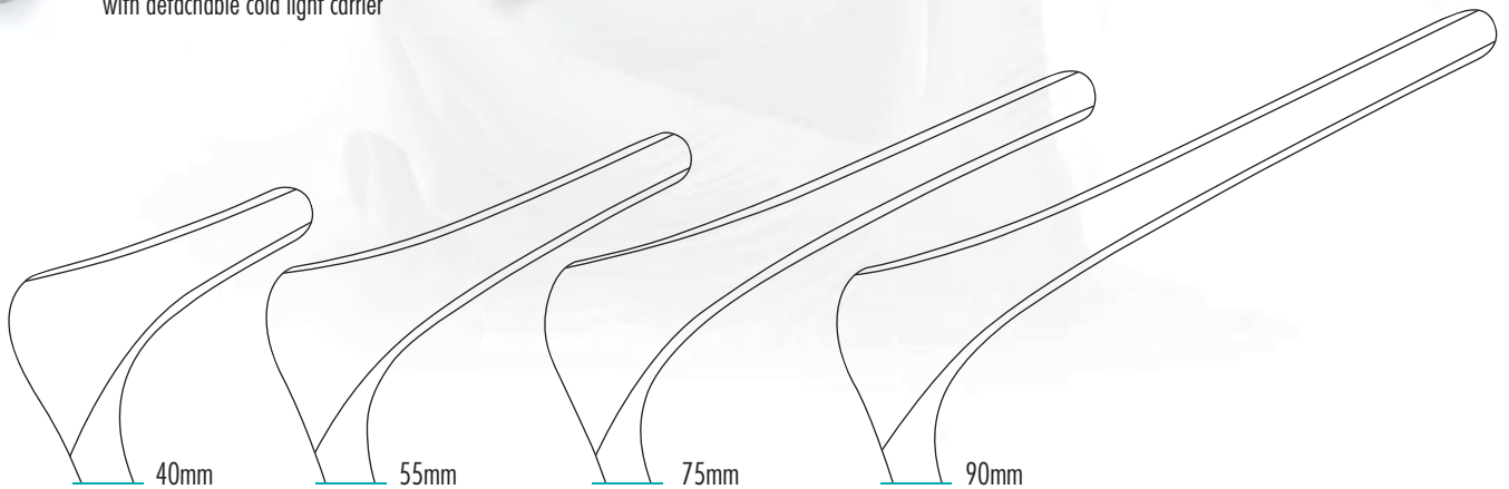
KILLIAN Nasal Speculum, aseptic joint, with detachable cold light carrier
